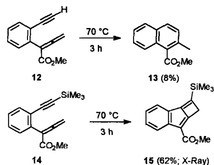
Scheme 9. Gillmann's reported formal [2+2] cycloaddition.
