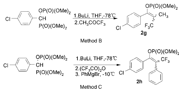
SCHEME 2 Methods B and C.
