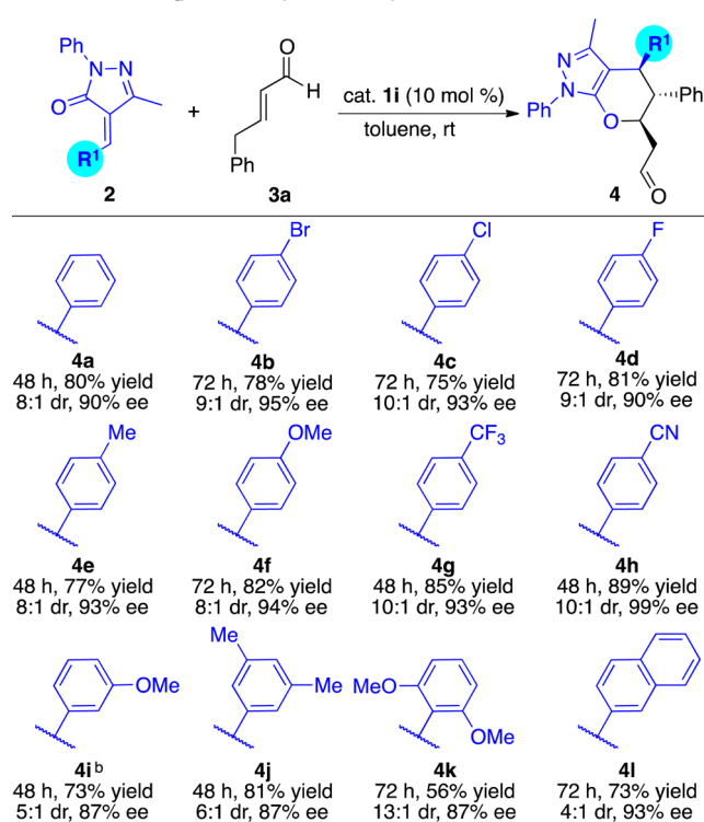
Scheme 2. Scope of Alkylidene Pyrazolones a
