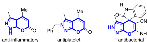
Figure 1. Some biologically active pyranopyrazol(on)es.
