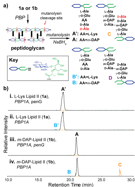
Figure 2. The m -DAP residue in Lipid II is essential for transpeptidase-catalyzed cross-linking. (a) Schematic of method for analyzing PG synthesis by PBPs. 14 (b) LC/MS extracted chromatograms of PBP1A and L-Lys Lipid II ( 1a ) reactions produce only A', representing unmodified polymer, in the presence of the inhibitor penG (i), but both A' and B', representing hydrolyzed peptide side chain, without penG (ii). PBP1A and m -DAP-Lipid II ( 1b ) reactions reveal fragment C in addition to fragments A and B, indicating the formation of cross-linked PG (iv); no cross-links are formed in the presence of penG (iii). The PGT inhibitor moenomycin prevented formation of all fragment peaks (Figure S1). For chromatograms (i, ii): (M+2H)/2 ions corresponding to fragments A' and B' were extracted: A': 485.2; B': 449.7; masses corresponding to predicted cross-linked fragments were not observed. For chromatograms (iii, vi): (M+2H)/2 ions corresponding to fragments A–D were extracted: A: 507.2; B: 471.7; C: 968.9; D: 933.4.
