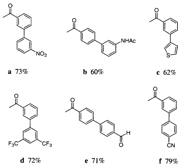
Figure 2. Synthesis of biarylic ketones 8 via Suzuki couplings onto vinyl ether 2 .
