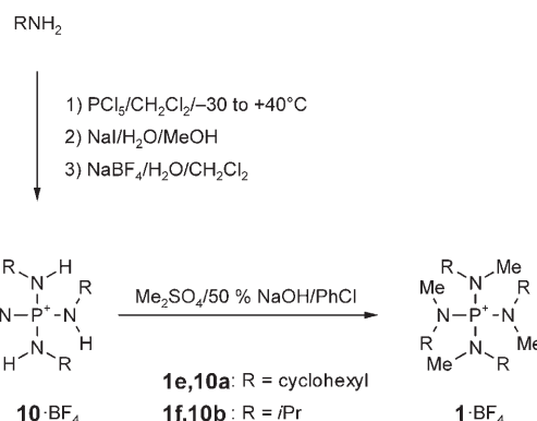
Scheme 6. Synthesis of 1e,f ·BF 4 .
