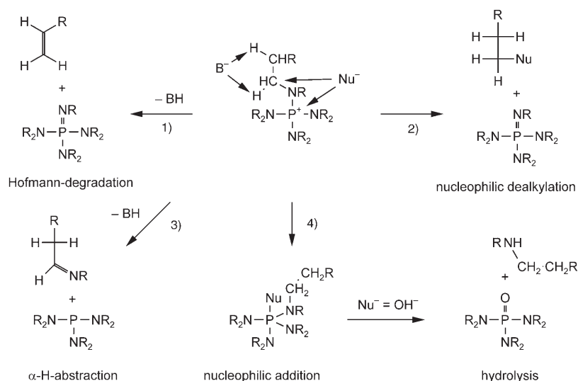
Scheme 1. Modes of decay of peralkylated tetraaminophosphonium cations (paths 1–4).
