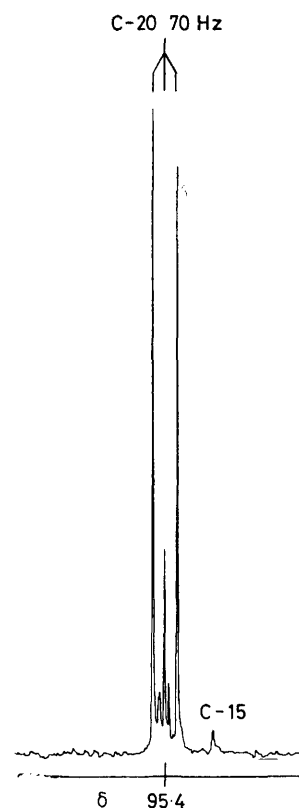
FIGURE 3 13 C N.m.r. signals from meso -bridges of [19,20- 13 C 2 ]-coproporphyrin-III tetramethyl ester [as (12)] in CDCl 3 containing Pr([ 2 H 5 ]) 3 fod 3
