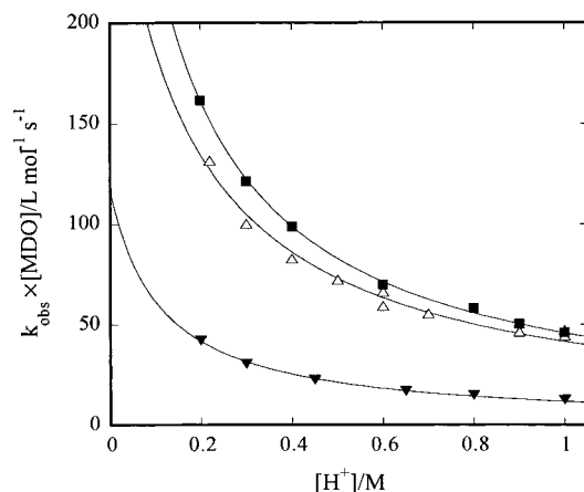
Figure 2. pH profiles for selected sulfenato complexes. The lines represent least-squares fitting to eq 9. Data are shown for complexes 1b (open triangles), 4b (filled triangles), and 6b (squares).
