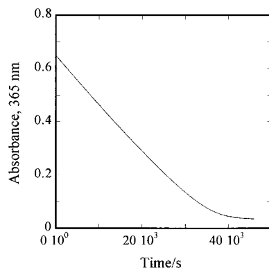
Figure 1. Absorbance–time recording of the reaction between (1b)–Cl 2 (1.0 mM) and H 2 P(O)OH (50 mM) catalyzed by CH 3 ReO 3 (84 μM). Conditions: 0.13 M HCl in 1:1 aqueous acetonitrile at 298 K.
