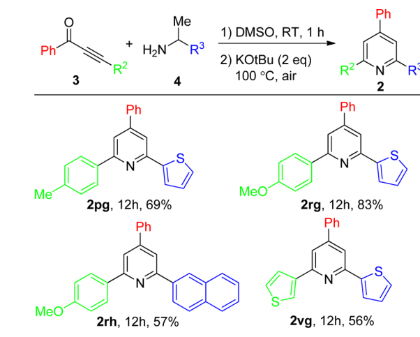
Scheme 4. One-Pot Synthesis of Unsymmetrical 2,4,6-Triarylpyridines
