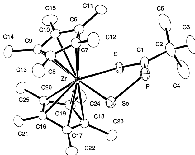
Fig. 3. Molecular structure of 11 together with selected bond lengths (Å) and bond angles ( ^\circ ): Zr–S 2.5440(6), Zr–Se 2.6385(3), S–C(1) 1.740(3), P–C(1) 1.709(3), Se–P(1) 2.2284(8), C(1)–C(2) 1.534(4), Zr–C(7) 2.584(2), Se–Zr–S 86.16(2), Zr–S–C(1) 105.97(9), S–C(1)–P 126.3(2), C(1)–P–Se 108.86(9), P–Se–Zr 97.66(2), P–C(1)–C(2) 117.6(2), C(8)–Zr–C(16) 94.47(8).
