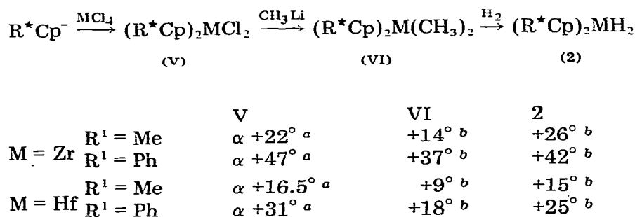
SCHÉMA 3. Solvant de mesure a = \text{CHCl}_3 , b = \text{C}_6\text{H}_6 , concentration 25 g/l; R^* = \text{R}^1 \text{CH}(\text{Et})\text{CH}_2 .
