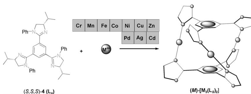
Figure 1. Schematic representation of the formation of the sandwich-shaped ( M )- [M_3(L_3)_2] complexes from ( S,S,S )- 4 and a series of different d^3 – d^{10} transition-metal ions.
