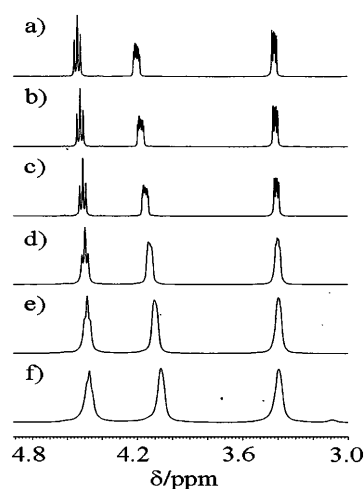
Figure 6. Variable-temperature ^1\text{H} NMR spectra of the [\text{Ag}_3(\text{L}_s)_2(\text{NO}_3)_3] complex ( (M) -8) (600 MHz, \text{CD}_2\text{Cl}_2 ): a) 293 K, b) 273 K, c) 253 K, d) 233 K, e) 213 K, and f) 193 K.
