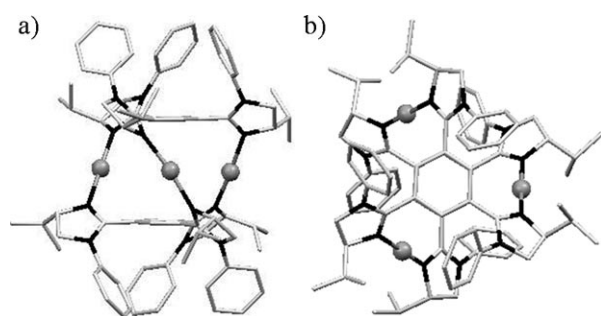
Figure 5. Crystal structure of (M) - [\text{Ag}_3(\text{L}_s)_2(\text{NO}_3)_3] ( (M) -8). a) side view, and b) top view. Color code: C (light gray), N (black), Ag (dark gray). H and \text{NO}_3^- were omitted for clarity.
