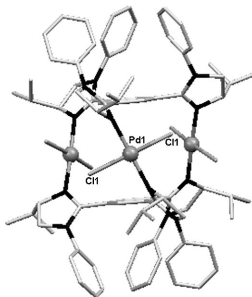
Figure 7. Crystal structure of (M) - [\text{Pd}_3(\text{L}_s)_2\text{Cl}_6] ( (M) -9). Color code: C (light gray), N (black), Pd (dark gray), and Cl (gray). All hydrogen atoms have been omitted for clarity.
