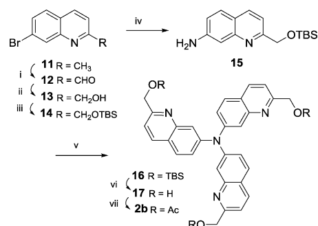
Scheme 2. Synthesis of 2b . Reagents and conditions: i) \text{SeO}_2 (1.3 equiv), dioxane, 80^\circ\text{C} , 3 h (95%); ii) \text{NaBH}_4 (1.1 equiv), EtOH, RT, 1 h (78%); iii) TBSCl (1.2 equiv), imidazole (1.2 equiv), DMF, RT, 3 h (64%); iv) CuI (0.2 equiv), L-proline (0.4 equiv), \text{K}_2\text{CO}_3 (3.0 equiv), aq. \text{NH}_4\text{OH} (28%, 10 equiv), DMSO, 80^\circ\text{C} , 18 h (35%); v) 14 (2.2 equiv), [\text{Pd}_2(\text{dba})_3] (0.2 equiv), t\text{BuONa} (2.2 equiv), t\text{Bu}_3\text{P} (1 m in toluene, 0.8 equiv), toluene, 110^\circ\text{C} , 18 h (83%); vi) HF–pyridine (7.5 equiv), MeCN, RT, 1 h (85%); vii) \text{Ac}_2\text{O} (4.5 equiv), \text{Et}_3\text{N} (4.5 equiv), DMAP (cat), \text{CH}_2\text{Cl}_2 , RT, 2 h (88%).
