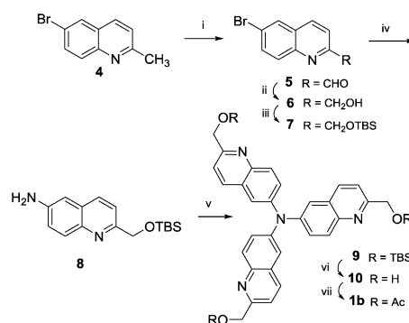
Scheme 1. Synthesis of 1b . Reagents and conditions: i) \text{SeO}_2 (1.3 equiv), dioxane, 80^\circ\text{C} , 3 h (97%); ii) \text{NaBH}_4 (1.1 equiv), EtOH, RT, 1 h (85%); iii) TBSCl (1.1 equiv), imidazole (1.1 equiv), DMF, RT, 3 h (80%); iv) CuI (0.2 equiv), L-proline (0.4 equiv), \text{K}_2\text{CO}_3 (3.0 equiv), \text{NH}_4\text{OH} (aq. 28%, 10 equiv), DMSO, 80^\circ\text{C} , 18 h (58%); v) 7 (2.2 equiv), [\text{Pd}_2(\text{dba})_3] (0.1 equiv), t\text{Bu}_3\text{P} (1 m in toluene, 0.2 equiv), t\text{BuONa} (2.4 equiv), toluene, 110^\circ\text{C} , 18 h (79%); vi) HF–pyridine (7.5 equiv), MeCN, RT, 1 h (70%); vii) \text{Ac}_2\text{O} (4.5 equiv), \text{Et}_3\text{N} (4.5 equiv), DMAP (cat), \text{CH}_2\text{Cl}_2 , RT, 2 h (89%).
