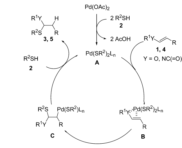
Scheme 3. A Possible Reaction Pathway of Pd-Catalyzed Hydrothiolation of Heteroatom-Substituted Alkenes
