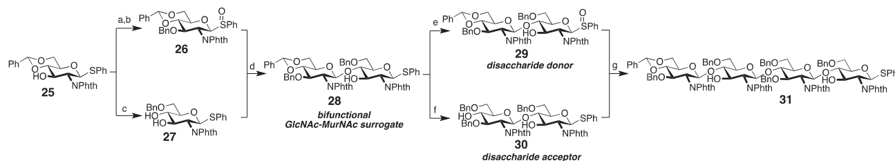
Scheme 5. Reagents and conditions: (a) BnBr (1.1 equiv), NaH (1.2 equiv), Bu 4 NI (0.1 equiv), DMF, rt, 70%; (b) mCPBA (1 equiv), CH 2 Cl 2 , –78 °C to rt, 88%; (c) HSiEt 3 (5 equiv), TFA (5 equiv), CH 2 Cl 2 , 0 °C, 93%; (d) 27 (1.5 equiv), ADMB (5 equiv), DTBMP (5 equiv), Tf 2 O (1 equiv), CH 2 Cl 2 , MS 4 Å, 58%; (e) mCPBA (1.1 equiv), CH 2 Cl 2 , 77%; (f) HSiEt 3 (12 equiv), BF 3 ·OEt 2 (2 equiv), CH 2 Cl 2 , 70%; (g) 29 (1.25 equiv), ADMB (6.25 equiv), DTBMP (3.75 equiv), Tf 2 O (1.25 equiv), CH 2 Cl 2 , MS 4 Å, 55%. Abbreviations: ADMB=4-allyl-1,2-dimethoxybenzene, DTBMP=2,6-di- tert -butyl-4-methylpyridine.
