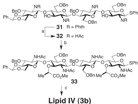
Scheme 6. Reagents and conditions: (a) ethylenediamine, EtOH/MeCN/THF, 60 °C, 48 h; then: Ac 2 O, MeOH/H 2 O, 70%; (b) NaH, DMF, S -2-bromopropionic acid, then: TMSCHN 2 , MeOH, PhH; 75%; (c) see Ref. 10m.
