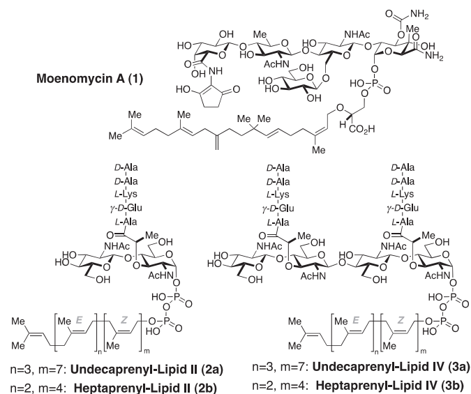
Fig. 1. Molecular structures of moenomycin A (1), lipid II (2), and lipid IV (3).
