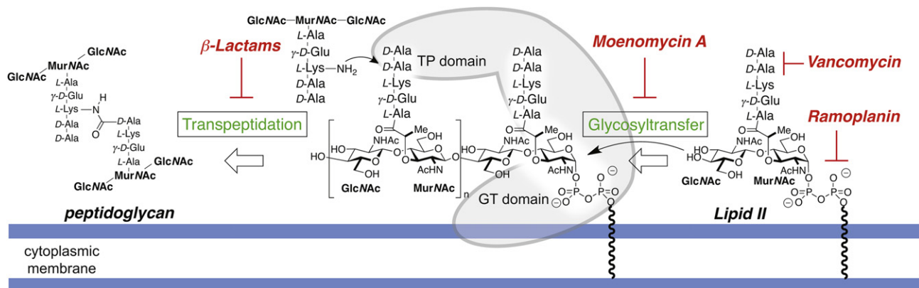
Scheme 1. The final stages of peptidoglycan biosynthesis involve polymerization of lipid II to make oligosaccharide chains followed by cross-linking via transpeptidation. This sequence is often performed by bifunctional enzymes containing distinct glycosyl transferase (GT) and transpeptidase (TP) domains (depicted in gray). Peptidoglycan synthesis can be disrupted at different steps by various antibiotics.
