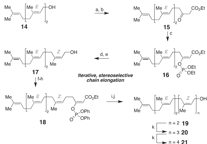
Scheme 3. Reagents and conditions: (a) \text{PBr}_3 (0.37 equiv), \text{Et}_2\text{O} , -30^\circ\text{C} to rt, 96%; (b) ethyl acetoacetate (2 equiv), NaH (2.2 equiv), BuLi (2.1 equiv), THF, 0^\circ\text{C} , 87%; (c) \text{ClPO}(\text{OEt})_2 (1.1 equiv), \text{NEt}_3 (1.1 equiv), DMAP (0.1 equiv), DMPU, 0^\circ\text{C} , 69%; (d) CuI (3 equiv), MeLi (3 equiv), MeMgCl (5 equiv) THF; (e) DIBAL-H (2.2 equiv), PhMe, 66% over two steps; (f) \text{PBr}_3 (0.37 equiv), \text{Et}_2\text{O} , -30^\circ\text{C} to rt; (g) ethyl acetoacetate (2 equiv), NaH (2.2 equiv), BuLi (2.1 equiv), THF, 0^\circ\text{C} , 70% (two steps); (h) \text{ClPO}(\text{OPh})_2 (2 equiv), \text{NEt}_3 (2 equiv), DMAP (0.2 equiv), DMPU, 0^\circ\text{C} , 86%; (i) MeMgCl (3 equiv), \text{Fe}(\text{acac})_3 (0.05 equiv), THF/NMP=20/1; (j) DIBAL-H (2.2 equiv), PhMe, 75% (two steps); (k) see f–j, 45–60% yield over five steps.
