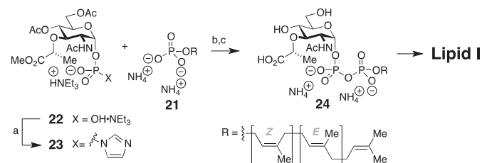
Scheme 4. Reagents and conditions: (a) CDI, DMF then MeOH; (b) N -Methylimidazole·HCl (4 equiv), DMF/THF 1/1, rt, 12 h; (c) 1 M LiOH·H 2 O, THF/MeOH/H 2 O (3:1:1), 54%.
