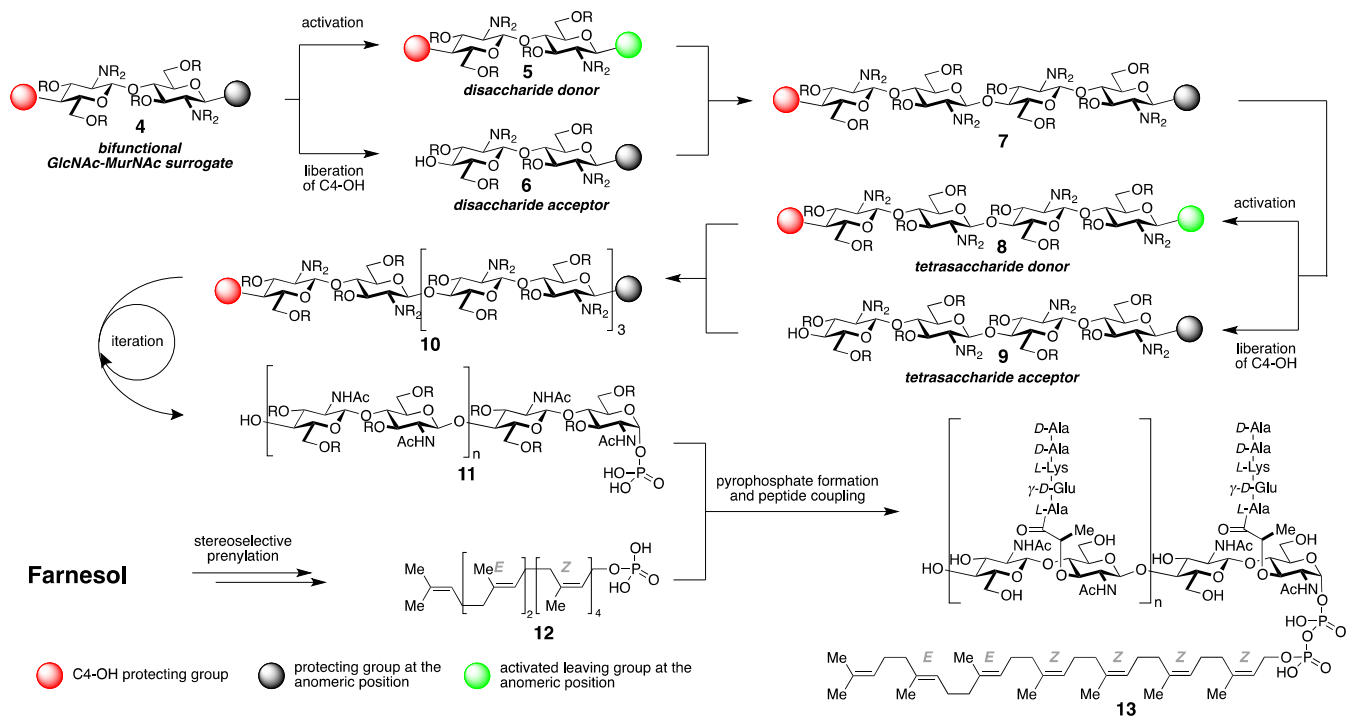
Scheme 2. Disaccharide 4 , equipped with a suitable C4–OH group (red dot) and an anomeric protecting group (black dot), gets converted into both a disaccharide donor ( 5 ) and acceptor ( 6 ). Coupling of 5 and 6 yields tetrasaccharide 7 that can be converted into octasaccharide 10 in a similar sequence via donor 8 and acceptor 9 . Repetition of this sequence followed by coupling to 12 allows access to diphospholipid oligosaccharides 13 with different length of the oligosaccharide.
