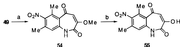
Scheme 5 a
