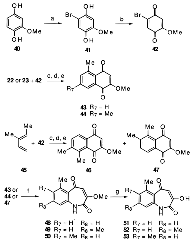
Scheme 4 a
