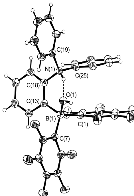
Fig. 2. Molecular structure of 1-[N(H)Ph 2 ]-2-[B(OH)(C 6 F 5 ) 2 ]C 6 H 4 ( 2 ) in the crystal.
