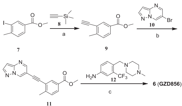
Scheme 1. Synthetic route of compound GZD856. Reagents and conditions: (a) i. \text{Pd}(\text{dppf})_2\text{Cl}_2 , CuI, \text{Et}_3\text{N} , DMF, 80^{\circ}\text{C} ; ii. \text{K}_2\text{CO}_3 , MeOH, rt, 90%; (b) \text{Pd}(\text{PPh}_3)_2\text{Cl}_2 , CuI, DIPEA, DMF, 80%; (c) t\text{-BuOK} , THF, -20^{\circ}\text{C} , 75%.
