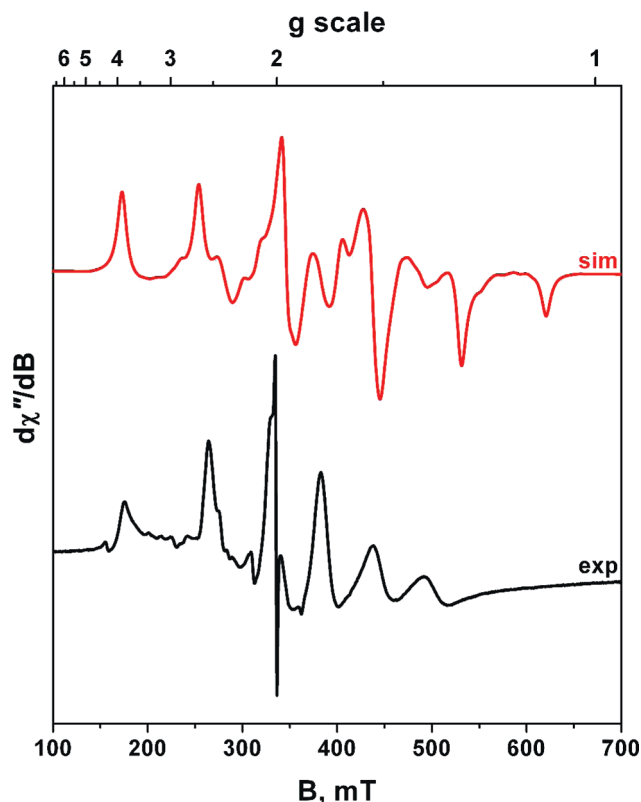
Figure 6. X-band EPR spectrum of 3d in \text{CH}_2\text{Cl}_2 at 20 K. The simulation is shown in red with the experimental spectrum in black (conditions: frequency, 9.41 GHz; power, 6.3 mW; modulation, 1.5 mT).
