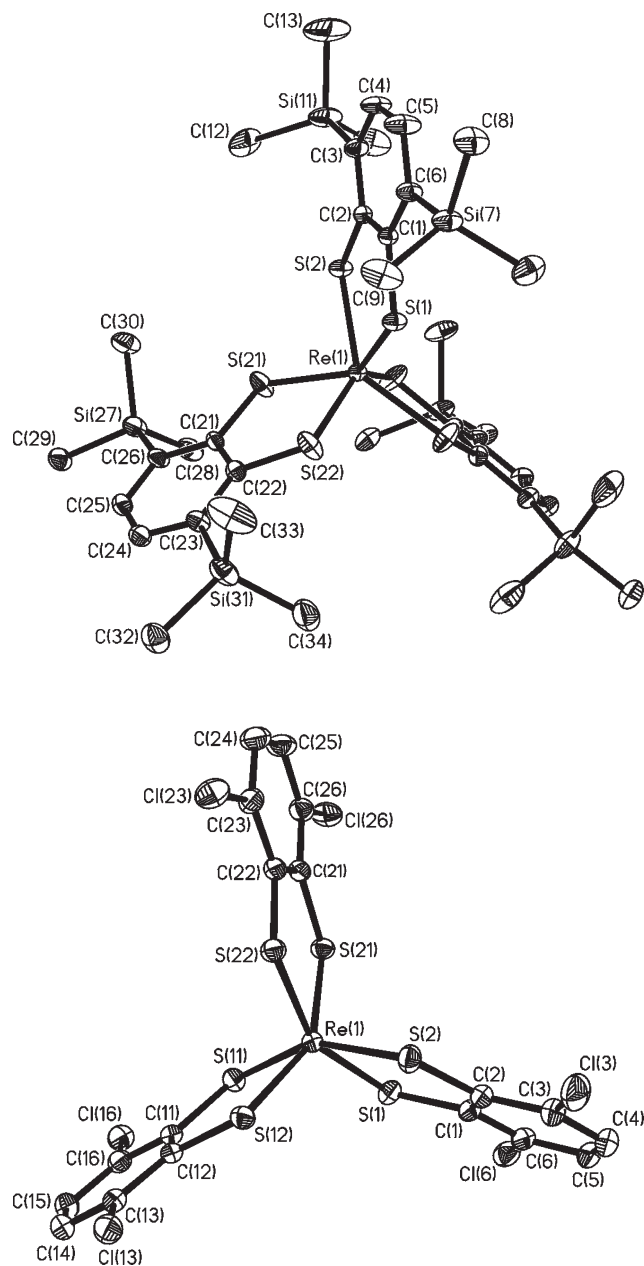
Figure 4. Structure of the monoanions in 1c (top) and 2c (bottom).
