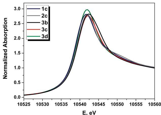
Figure 8. Normalized Re L_3 -edge XAS data of [\text{Re}(\text{tms})_3]^{1-} ( 1c ), [\text{Re}(\text{Cl}_2\text{-bdt})_3]^{1-} ( 2c ), [\text{Re}(\text{bdt})_3] ( 3b ), [\text{Re}(\text{bdt})_3]^{1-} ( 3c ), and [\text{Re}(\text{bdt})_3]^{2-} ( 3d ).
