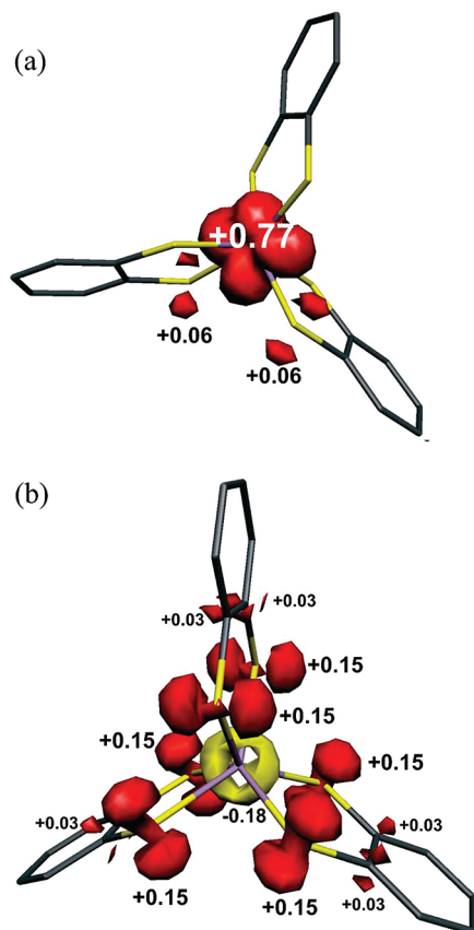
Figure 11. Spin density plots of (a) the dianion in 3d and (b) neutral 3b , from spin unrestricted DFT calculations together with values from the Mulliken analyses (red, \alpha -spin; yellow, \beta -spin). A complete Mulliken spin density listing is available in the Supporting Information.
