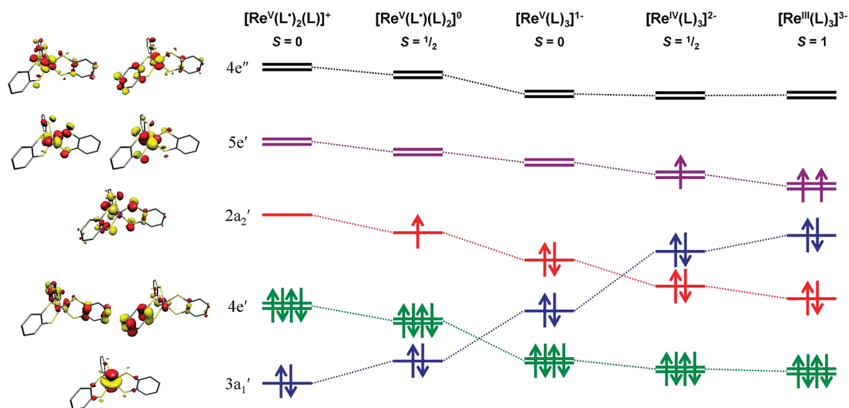
Figure 10. Qualitative MO scheme depicting the ordering of the frontier orbitals for the [\text{Re}(\text{L})_3]^z ( z = 1+, 0, 1-, 2-, 3- ) electron transfer series derived from B3LYP DFT calculations. The MOs shown on the left are derived from the [\text{Re}(\text{bdt})_3]^+ calculation with D_{3h} symmetry labels. 56
