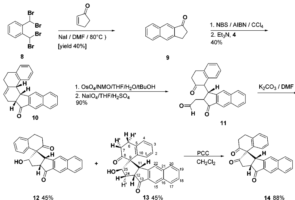
Scheme 2. Synthesis of Enhanced Model Compounds
