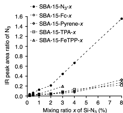
Figure 3. IR peak area of azide ( 2110 \text{ cm}^{-1} normalized to the signal at 1640 \text{ cm}^{-1} ) of the SBA-15- \text{N}_3\text{-}x and SBA-15-R- x materials as a function of the mixing ratio x of \text{Si-N}_3 .
