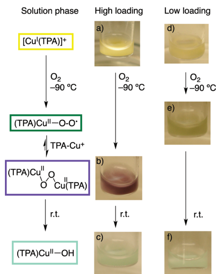
Figure 7. Color changes upon oxygenation of SBA-15-TPA-4 (a–c) and SBA-15-TPA-0.5 (d–f) with 0.9 equiv of [\text{Cu}^{\text{I}}(\text{MeCN})](\text{SbF}_6) in EtCN at -90^\circ\text{C} . Characteristic colors of intermediates in the corresponding homogeneous solutions are displayed to the left.
