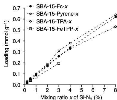
Figure 4. Loadings (mmol g -1 ) of SBA-15-R- x (R = Fc, pyrene, TPA, and FeTPP) as a function of the mixing ratio x of Si-N 3 . Fc and FeTPP loadings were determined by iron ICP analysis of digested samples. Pyrene and TPA loadings were determined by UV-vis spectrometry of digested samples.
