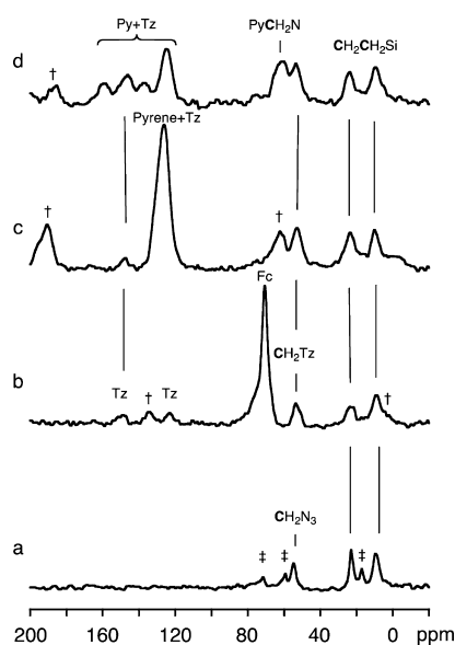
Figure 1. CP-MAS ^{13}\text{C} solid-state NMR of (a) SBA-15- \text{N}_3 -8, (b) SBA-15- \text{Fc} -8, (c) SBA-15-pyrene-8, and (d) SBA-15-TPA-8. (†): spinning sideband signals, (‡): residual \text{P}_{123} template and solvent \text{EtOH}/\text{EtO-Si} groups, (Fc): ferrocene ring, (Py): pyridine group, (Tz): triazole group.
