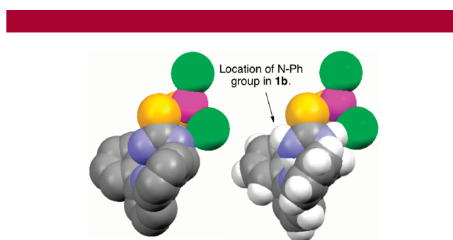
Figure 4. B98/LANL2DZ optimized lowest-energy structure for a minimal analogue of 1b ·HgCl 2 , without (left) and with (right) hydrogen atoms.
