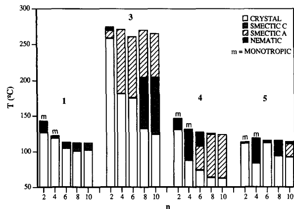
Fig. 3. Thermal behavior of compounds of types 1 , 3 , 4 and 5 .
