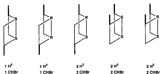
Fig. 1. Schematic representation of the possible diastereomers for the 2-bromopropionic-bridged complexes. The bar indicates the N-C 6 H 4 -OR moiety. R or S indicates the conformation of the carboxylate ligand in that position. The number of H 3 or CHBr NMR signals predicted for each isomer are given under the structure.
