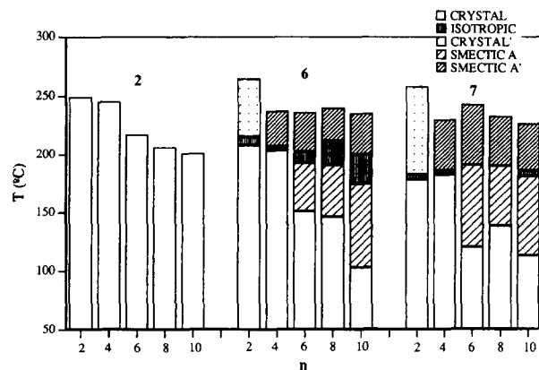
Fig. 4. Thermal behavior of compounds of types 2 , 6 and 7 . Smectic A' is used to label the second S A phase produced on heating.
