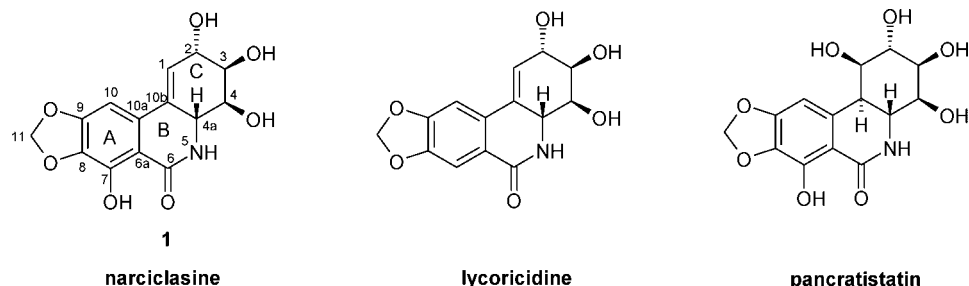
Figure 1. Chemical structures of narciclasine, lycoricidine, and pancratistatin.
