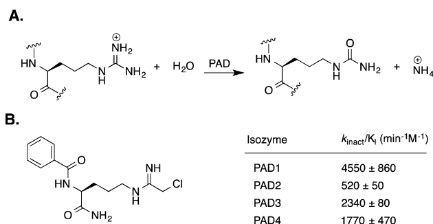
Figure 1. (A) Transformation catalyzed by PADs. (B) Cl-amidine, one of the most advanced PAD inhibitors. 16
