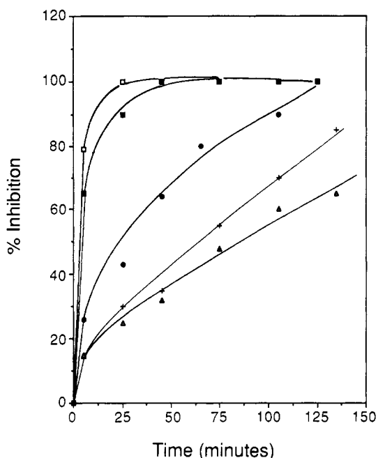
Figure 3. Inhibition of horse serum cholinesterase by bis(2,2-dimethylaziridinyl)phosphinyl nucleosides: 5, ■; 6, □; 14, +; 15, △; AB-132 (standard), ●.
