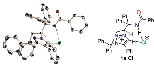
Figure 1. ORTEP diagram of 1a ·Cl (calculated hydrogens and solvent molecules are omitted for clarity).
