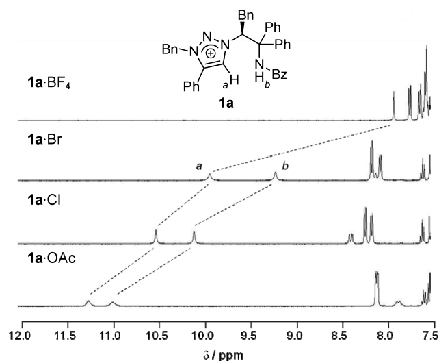
Figure 2. Partial ^1\text{H} NMR spectra of 1a ·BF 4 , 1a ·Br, 1a ·Cl, and 1a ·OAc in CD 2 Cl 2 (0.01 M) at 293 K.
