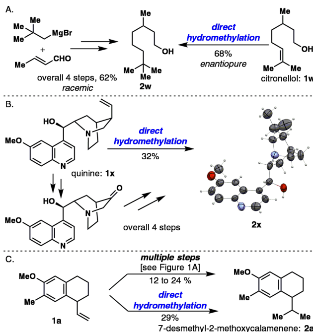
Figure 3. Direct hydromethylation as a step-economic method.
