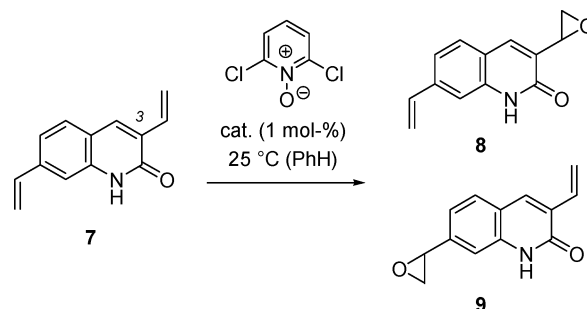
Scheme 3. Regio- and Enantioselective Epoxidation of Diolefin 7 to Product 8 (See the Text for Further Explanation)
