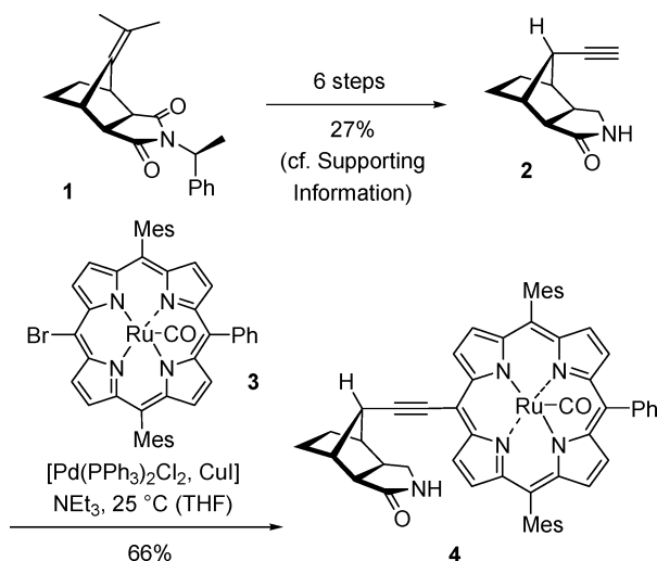
Scheme 1. Preparation of Chiral Ruthenium Porphyrin Complex 4 from Substrate 1
