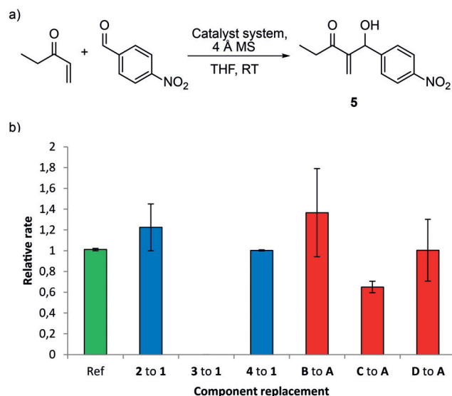
Figure 2. a) Model MBH reaction. b) Observed initial rate difference for MBH reaction upon selective replacement of investigated components 2–4 or B–D by equivalent amount of non-functionalized analogues 1 or A in the pre-generated catalyst system. Conditions: 0.12 mmol p -nitrobenzaldehyde, 0.24 mmol ethyl vinyl ketone, 4 Å MS (300 mg), anhydrous THF (0.5 mL), pre-generated imine catalyst system (0.075 mmol of each initial component A–D and 1–4 except for the omitted building block and the replacement compound A or 1 of which 0.15 mmol was added). Duplicate experiments; for further experimental details and kinetic plots, see the Supporting Information.
