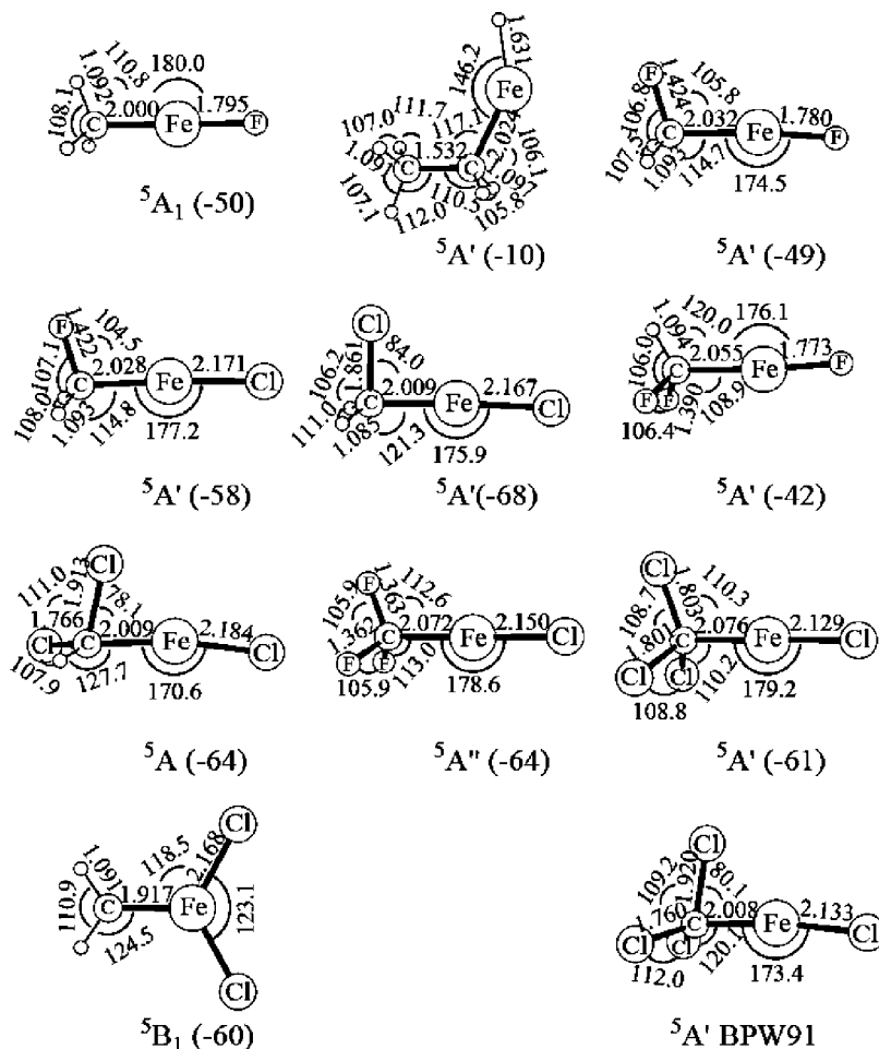
Figure 9. Optimized molecular structures of Fe insertion complexes in the ground quintet states. The structures were calculated with B3LYP/6-311++G(3df,3pd), except for the \text{CCl}_3\text{--FeCl} structure, which was calculated with BPW91/6-311++G(3df,3pd). \text{CH}_3\text{--FeF} has a C_{3v} structure, whereas \text{CHCl}_2\text{--FeCl} has a C_1 structure. Others have C_s structures. The bond lengths and angles are in Å and deg, respectively. The product energy relative to Fe and the parent molecule is given in kcal/mol.
