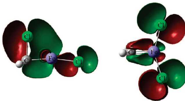
Figure 11. Molecular orbital for the CH 2 Cl–FeCl insertion complex showing the chlorine lone pair–iron interaction, which leads to \alpha -Cl transfer and the CH 2 =FeCl 2 methyldene complex, also illustrated.
