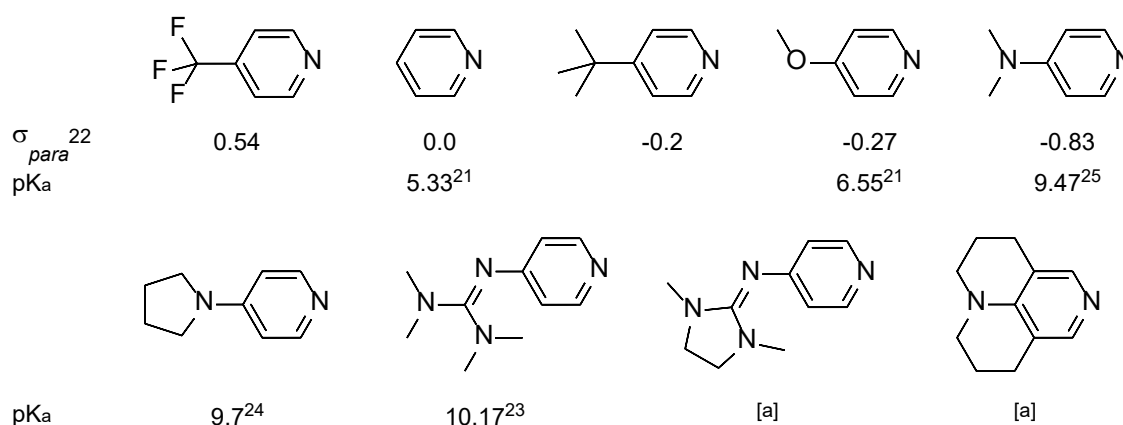
Figure 3: Pyridine derivatives used for ligand synthesis together with Hammett constants and reported pK_a values of the corresponding acids. The donor strength increases from left to right. [20, 22-24] [a]: To the best of our knowledge no experimental pK_a value is available in literature.
