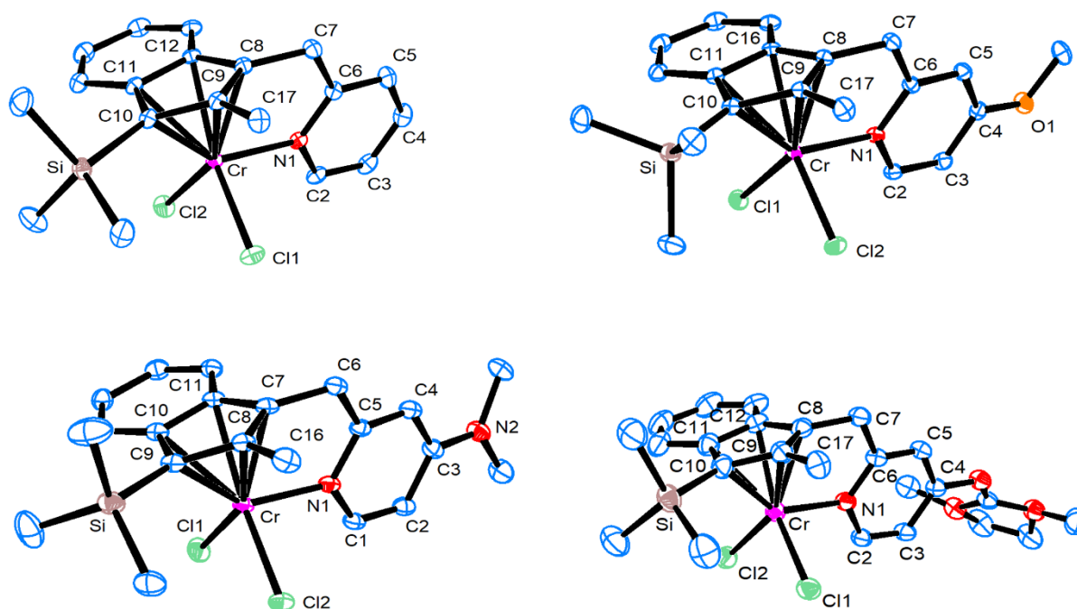
Figure 5: Molecular structures as obtained from x-ray diffraction of complexes 2 , 4 , (top) 5 , 6 (bottom, from left to right). Blue: C, red: N, green: Cl, purple: Cr, beige: Si, orange: O. H atoms and solvent molecules are omitted for clarity. Displacement ellipsoids are drawn with 50% probability. For details of crystal structure analysis see Supporting Information.
