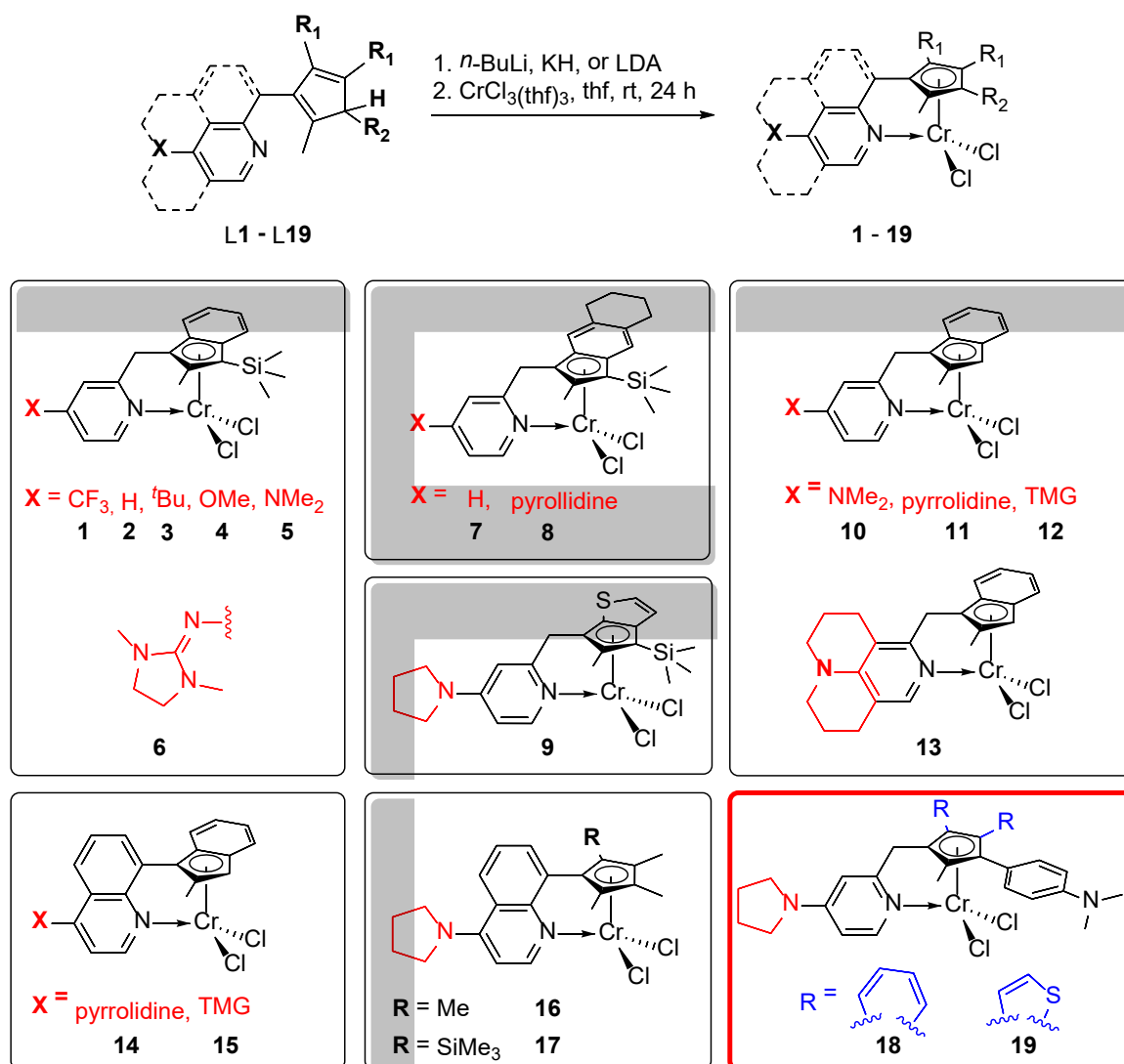
Scheme 3: Synthetic procedure and illustration of the new complexes 1-19 . The complexes are grouped by structural similarity. Complexes 18 and 19 showed the highest activity for indenyl and cp complexes of this type so far.
