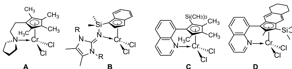
Figure 1: Examples of chromium pre-catalysts with N-donor functionalized cyclopentadienyl ligands.
