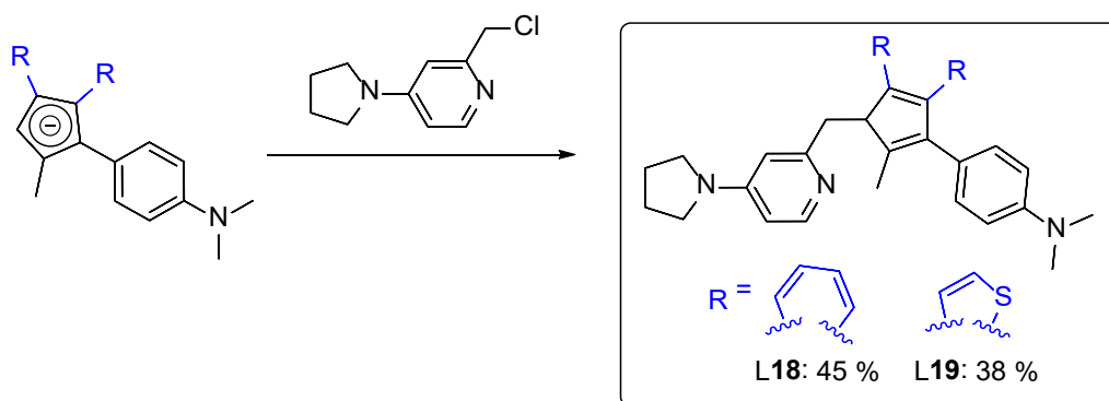
Scheme 2: Synthetic procedure for the ligands L18 and L19 with an N,N-dimethylaniline group.
