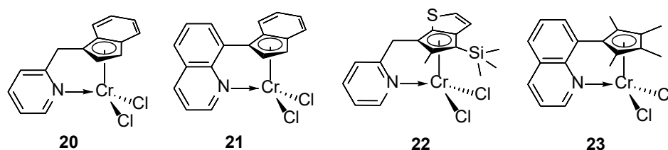
Figure 4: Literature known catalysts without 4-donor substituents used as reference. [2, 36-37]
