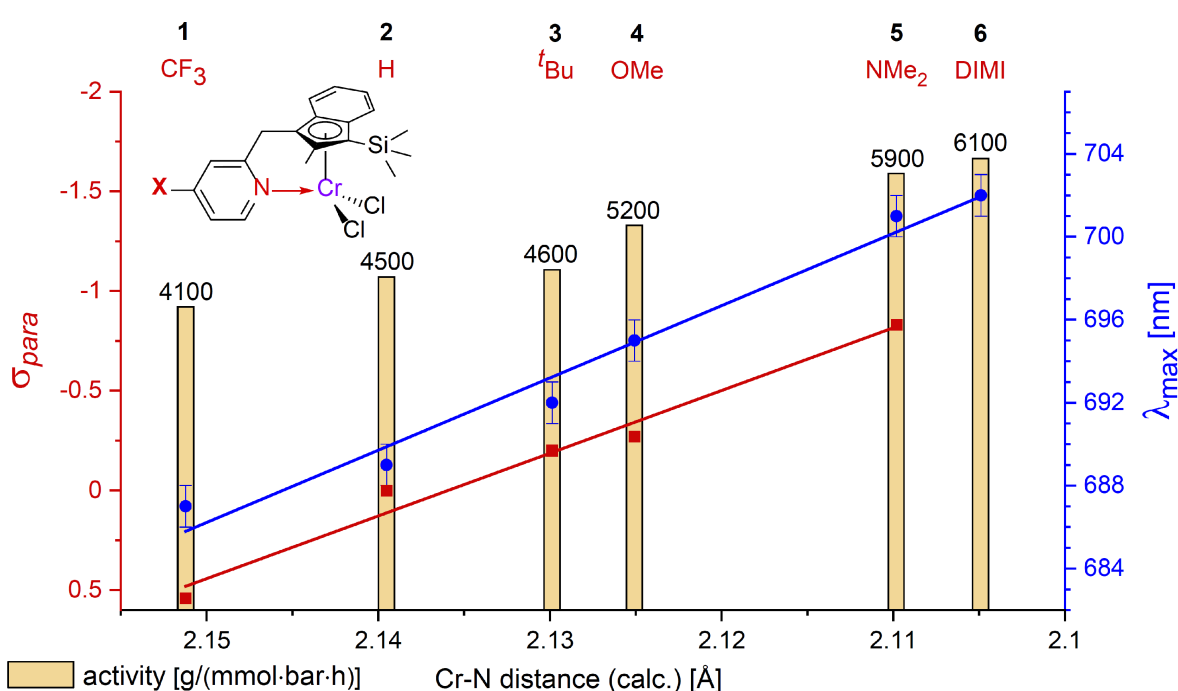
Figure 7: Plot of the calculated Cr-N distance vs. Hammett constant \sigma and the maximum of absorption spectra \lambda_{\max} of complexes 1 , 2 , 3 , 4 , 5 , 6 (from left to right). Corresponding catalytic activities are given as coloured bars. No \sigma -value for 6 was available in literature. DIMI = dimethylimidazolidine-imine.
