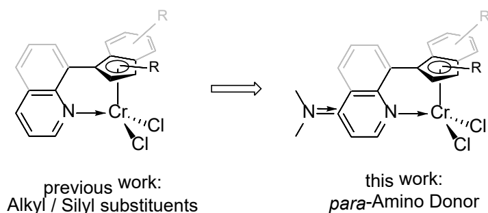
Figure 2: Previous and actual work on the influence of substituents.
