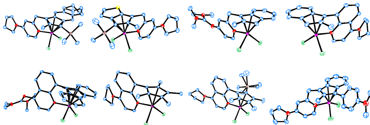
Figure 6: Molecular structures of complexes, 8 , 9 , 12 , 14 (upper line, from left to right) and 15 – 18 (lower line, from left to right). Blue: C, red: N, green: Cl, purple: Cr, brown: Si, yellow: S. H atoms and solvent molecules are omitted for clarity. Only one of two independent molecules is shown for complexes 17 and 18 . Displacement ellipsoids are drawn with 50% probability. For details of the crystal structure analysis see the Supporting Information.
