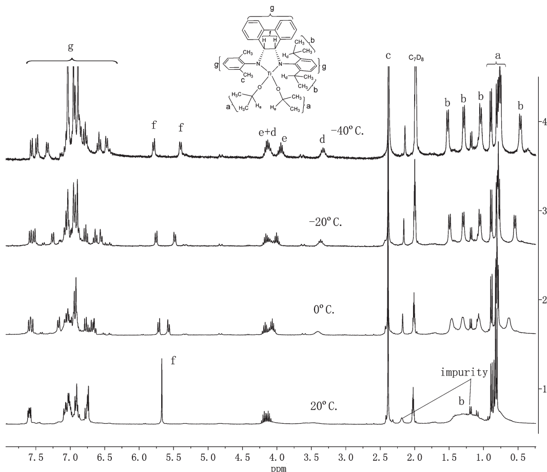
Figure 1. Variable-temperature ^1\text{H} NMR spectra of 2e in toluene- d_8 at +20, 0, -20 , and -40 ^\circ\text{C} .
