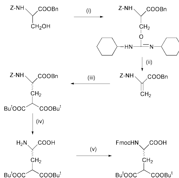
Scheme 1 Reagents and conditions: (i) DCC, \text{CH}_2\text{Cl}_2 (ii) \text{CuCl} (iii) di- tert -butyl malonate, NaH, DMF (iv) \text{H}_2 , Pd/C, MeOH (v) Fmoc-Cl, \text{NaHCO}_3 , 1,4-dioxane.
