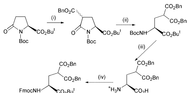
Scheme 3 Reagents and conditions: (i) \text{BnO}_2\text{C} , LDA, THF, -78^\circ\text{C} (ii) \text{BnOH} , \text{BnONa} (iii) \text{HCl} , \text{EtOAc} (iv) \text{Fmoc-OSu} , DIPEA.
