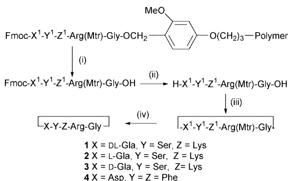
Scheme 2 (a) X^1 = \text{DL-Gla}(\text{OBu}^t)_2 , Y^1 = \text{Ser}(\text{Bu}^t) , Z^1 = \text{Lys}(\text{Boc}) ; (b) X^1 = \text{L-Gla}(\text{OBn})_2 , Y^1 = \text{Ser}(\text{Bu}^t) , Z^1 = \text{Lys}(\text{Boc}) ; (c) X^1 = \text{L-Gla}(\text{OBu}^t)_2 , Y^1 = \text{Ser}(\text{Bu}^t) , Z^1 = \text{Lys}(\text{Boc}) ; (d) X^1 = \text{D-Gla}(\text{OBu}^t)_2 , Y^1 = \text{Ser}(\text{Bu}^t) , Z^1 = \text{Lys}(\text{Boc}) ; (e) X^1 = \text{L-Asp}(\text{OBu}^t) , Y^1 = Z^1 = \text{Phe} . Reagents and conditions: (i) 1% TFA (ii) 10% piperidine-DMF (iii) EDC, DMAP, N -methylmorpholine for Schemes 2(a), 2(b) and 2(e), HATU, DIPEA, DMF, \text{CH}_2\text{Cl}_2 for Schemes 2(c) and 2(d) (iv) TFA.
