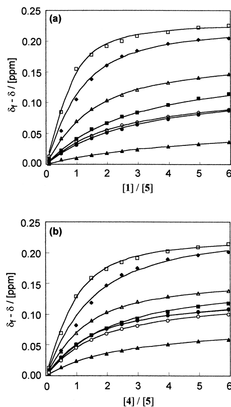
Fig. 4. ^1\text{H} -NMR Titration of 1 with 5 (a), 4 with 5 (b) at 24^\circ\text{C} in \text{CDCl}_3
