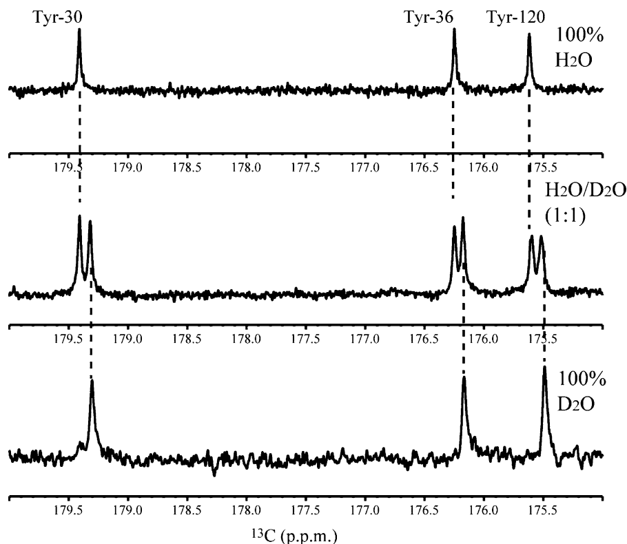
Figure 3. DEALS experiment for the carbonyl carbon ^{13}\text{C} NMR signals of the Tyr residues of EPPIb to monitor the amide deuterium–hydrogen exchange rates of the Cys residues. In order to monitor the amide exchange rates for Cys-31 and Cys-121, the carbonyl carbon NMR signals of the N-terminal neighbors of the two residues, namely Tyr-30 and Tyr-120, should be observed. For the DEALS experiment, EPPIb was dissolved in \text{H}_2\text{O}/\text{D}_2\text{O} (1:1) to observe the two-bond deuterium isotope shift effect. The fractionation factors ( [\text{D}]/[\text{H}] ) for the amides of Cys-31 and Cys-121 were estimated by the relative peak heights of the two isotope-shifted signals to be 0.9 and 1.0, respectively, which were identical with those obtained by the \text{C}_\beta signals (Table 2).
