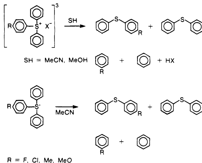
Scheme IV. Products from Photodecomposition by Triplet Energy Transfer and Electron-Transfer Sensitization of Sulfonium Salts
