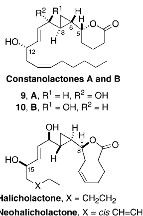
FIGURE 2. Cyclopropane-containing \text{C}_{20} oxylipins.
