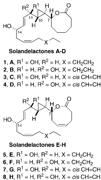
FIGURE 1. Shin's structural assignments to solandelactones A–H.
