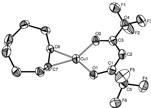
Figure 3. View of the molecular structure of [\text{Cu}(\text{hfacac})(\text{coe})] with the atomic numbering scheme.
