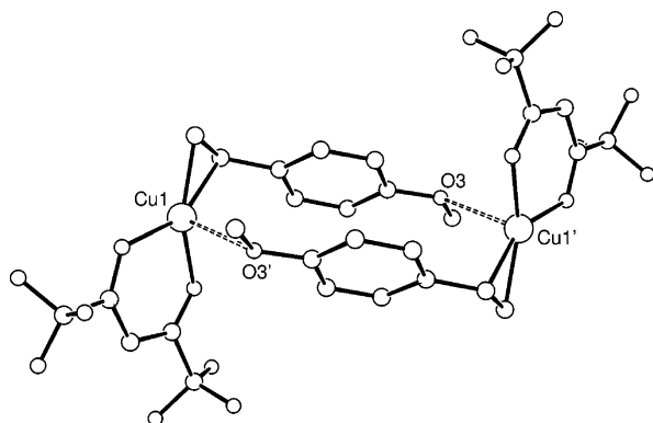
Figure 5. Schematic view of the centrosymmetric [Cu(hfacac)(van)] 2 dimeric units. Dashed lines indicate intermolecular contacts between copper and ethereal oxygen in adjacent molecules.
