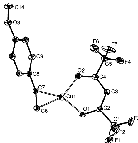
Figure 4. View of the molecular structure of [\text{Cu}(\text{hfacac})(\text{van})] with the atomic numbering scheme.
