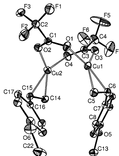
Figure 2. View of the molecular structure of [\text{Cu}(\mu\text{-CF}_3\text{COO})(\text{van})]_2 \cdot \text{C}_7\text{H}_8 with the atomic numbering scheme.
