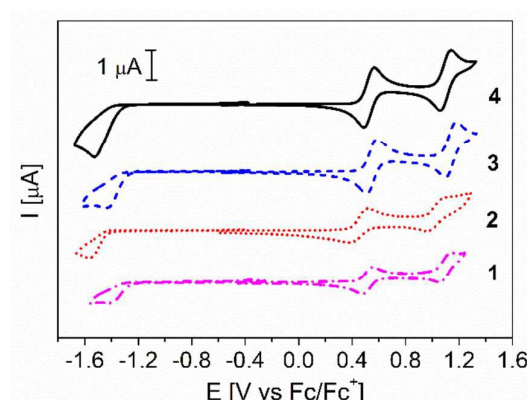
Figure 3. Cyclic voltammograms of oligomers 1-4 in ( 1 \times 10^{-3} mol L -1 in dichloromethane/ n -Bu 4 NPF 6 as supporting electrolyte). All scan rates were 100 mV s -1 and the potentials were internally referenced to the Fc/Fc + couple.
