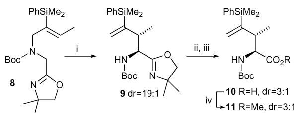
Scheme 2 Reagents and conditions: (i) n -BuLi, Et 2 O-HMPA (1 : 4), -78 to -40 °C, 14 h, 75% conversion; (ii) p -MePhSO 3 Me, 80 °C; (iii) 15% aq. NaOH, rt, 99% (2 steps); (iv) CH 3 N 2 , CH 2 Cl 2 , rt, 83%.
