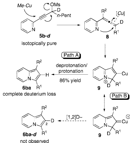
Scheme 1. Proposed Mechanism for Cascade Cyclization
