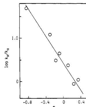
Figure 5. Hammett plot vs. \sigma for substituted N,N -dimethylanilines in the quenching reaction of ^1O_2 .
