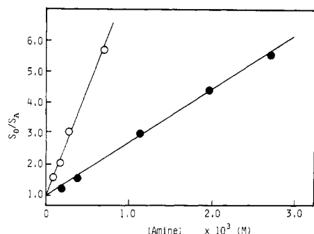
Figure 4. Plots of S_0/S_A vs. amine concentration. (●) for DMA and (O) for TMPD.
