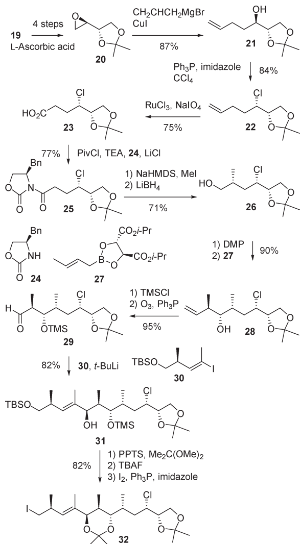
Scheme 4. Synthesis of the C Fragment
