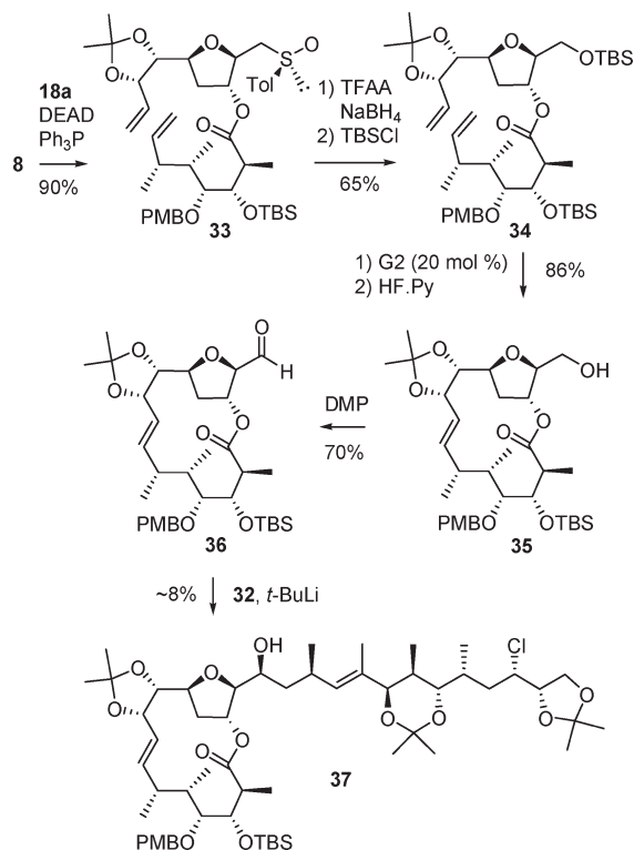
Scheme 5. Synthesis of the Macrolactone Intermediates
