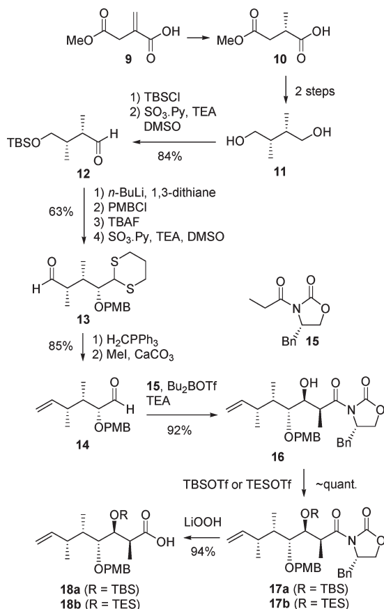
Scheme 3. Synthesis of the B Fragment
