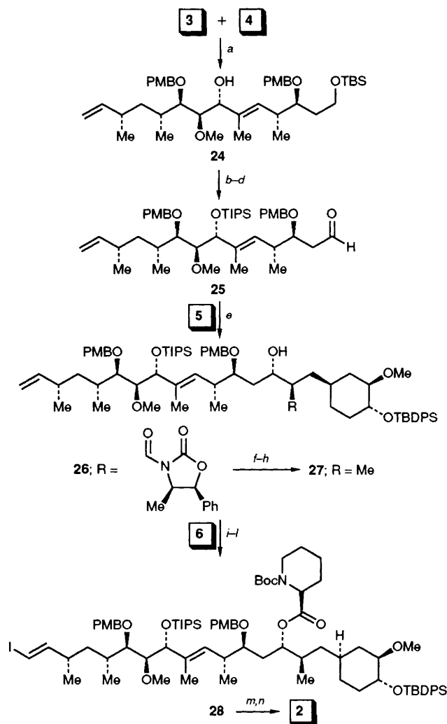
Scheme 5 Synthesis of key intermediate 2 . Reagents and conditions: (a) 3 (1.0 equiv.), 4 (2.5 equiv.), CrCl 2 (containing 0.1% NiCl 2 ) (10 equiv.), DMSO, 25 °C, 12 h, 87% (based on 10% recovered aldehyde); (b) TIPSOTf (1.5 equiv.), 2,6-lutidine (3 equiv.), CH 2 Cl 2 , 0 °C, 15 min., 98%; (c) HF-pyridine, THF, 25 °C, 3 h, 97%; (d) (COCl) 2 (1.5 equiv.), DMSO (3.2 equiv.), Et 3 N (5 equiv.), CH 2 Cl 2 , -78 to -10 °C, 1 h, 96%; (e) 5 (2.0 equiv.), Bu 3 BOTf (2.3 equiv.), Et 3 N (2.6 equiv.), CH 2 Cl 2 , -78 to 0 °C, 1 h then 24 (1 equiv.), -78 to 25 °C, 3 h, 95%; (f) LiBH 4 (2.2 equiv.), H 2 O (2.2 equiv.), Et 2 O, 0 °C, 1 h, 98%; (g) TsCl (2 equiv.), Et 3 N (4 equiv.), DMAP (0.2 equiv.), CH 2 Cl 2 , 25 °C, 24 h, 90% (based on 10% recovered diol); (h) LiEt 3 BH (10 equiv.), THF, 0 °C, 2 h, 91%; (i) N -Boc-L-pipecolic acid ( 6 ) (5 equiv.), diisopropylcarbodiimide (5 equiv.), diisopropylethylamine (1 equiv.), 4-pyrrolidinopyridine (0.5 equiv.), CH 2 Cl 2 , 0 °C, 4 h, 85%; (j) OsO 4 (0.2 equiv.), N -methylmorpholine N -oxide (3.5 equiv.), acetone-H 2 O (2:1), 25 °C, 12 h; (k) Pb(OAc) 4 (2.4 equiv.), Na 2 CO 3 (3 equiv.), C 6 H 6 , 0 to 25 °C, 15 min., 75% from olefin; (l) CHI 3 (4 equiv.), CrCl 2 (12 equiv.), THF-dioxane (4:1), 25 °C, 1 h, 94%; (m) DDQ (3 equiv.), CHCl 3 -H 2 O (19:1), 25 °C, 1 h, 98%; (n) TESOTf (15 equiv.), 2,6-lutidine (20 equiv.), CH 2 Cl 2 , 0 °C, 1 h then silica gel, CH 2 Cl 2 , 25 °C, 6 h, 94%.
