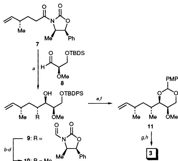
Scheme 2 Synthesis of key intermediate 3 . Reagents and conditions: (a) 7 (1 equiv.), Bu 2 BOTf (1.15 equiv.), Et 3 N (1.3 equiv.), CH 2 Cl 2 –78 to 0 °C, 1 h, then 8 (1 equiv.), –78 to 25 °C, 3 h, 85%; (b) LiBH 4 (2.2 equiv.), H 2 O (2.2 equiv.), Et 2 O, 0 °C, 1 h, 98%; (c) TsCl (1.2 equiv.), pyridine, 0 °C, 6 h, 90% (based on 20% recovered starting material); (d) LiEt 3 BH (5 equiv.), THF, 0 to 25 °C, 12 h, 92%; (e) Bu 4 NF (1.5 equiv.), THF, 0 to 25 °C, 1 h, 93%; (f) p -methoxybenzaldehyde dimethyl acetal (1.3 equiv.), CSA (0.2 equiv.), CH 2 Cl 2 , 25 °C, 4 h, 95%; (g) DIBAL (2 equiv.), CH 2 Cl 2 , –78 to 25 °C, 1 h, 98%; (h) (COCl) 2 (1.5 equiv.), DMSO (3.2 equiv.), Et 3 N (5 equiv.), CH 2 Cl 2 , –78 to –10 °C, 1 h, 96%.
