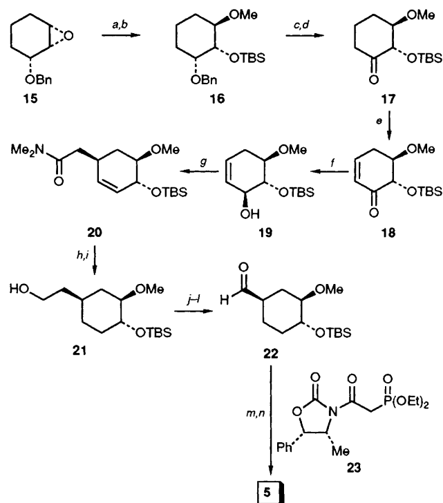
Scheme 4 Synthesis of key intermediate 5 . Reagents and conditions: (a) CSA (0.25 equiv.), MeOH, 25 °C, 2 h, 88%; (b) TBSOTf (1.5 equiv.), 2,6-lutidine (2 equiv.), CH 2 Cl 2 , 0 °C, 15 min., 98%; (c) 20% Pd(OH) 2 /C, H 2 , EtOH, 25 °C, 2 h, 95%; (d) (COCl) 2 (1.5 equiv.), DMSO (3.2 equiv.), Et 3 N (5 equiv.), CH 2 Cl 2 , -78 to -10 °C, 1 h, 92% (e) LDA (1.1 equiv.), TMSCl (1.1 equiv.), THF, -78 °C, 0.5 h then Pd(OAc) 2 (1.1 equiv.), MeCN, 50 °C, 18 h, 88%; (f) LiBH 4 (4 equiv.), CeCl 3 ·7H 2 O (2 equiv.), MeOH-THF (1:1), -78 °C, 0.5 h, 95%; (g) N,N -dimethylacetamide dimethyl acetal (5 equiv.), xylene, reflux, 24 h, 89%; (h) LiEt 3 BH (2.2 equiv.), THF, 0 to 25 °C, 2 h, 92%; (i) 10% Pd/C, H 2 , EtOH, 25 °C, 2 h, 96%; (j) o -NO 2 C 6 H 4 SeCN (1.2 equiv.), Bu 3 P (1.2 equiv.), THF, 0 to 25 °C, 2 h, 93%; (k) H 2 O 2 (30% aq.), THF, 0 to 25 °C, 2 h, 86%; (l) O 3 , CH 2 Cl 2 -MeOH (1:1, -78 °C, then Me 2 S, -78 to 25 °C, 6 h, 92%; (m) 23 (1.5 equiv.), LiCl (1.7 equiv.), diisopropylethylamine (1.7 equiv.), MeCN, 25 °C, 4 h, 96% (n) Rh(PPh 3 ) 3 Cl (0.05 equiv.), Et 3 SiH, 50 °C, 2 h then aq. HF in MeCN (10%), 0 °C, 2.5 h followed by TBDPSCl (1.5 equiv.), imidazole (3 equiv.), DMF, 25 °C, 6 h, 75% overall.
