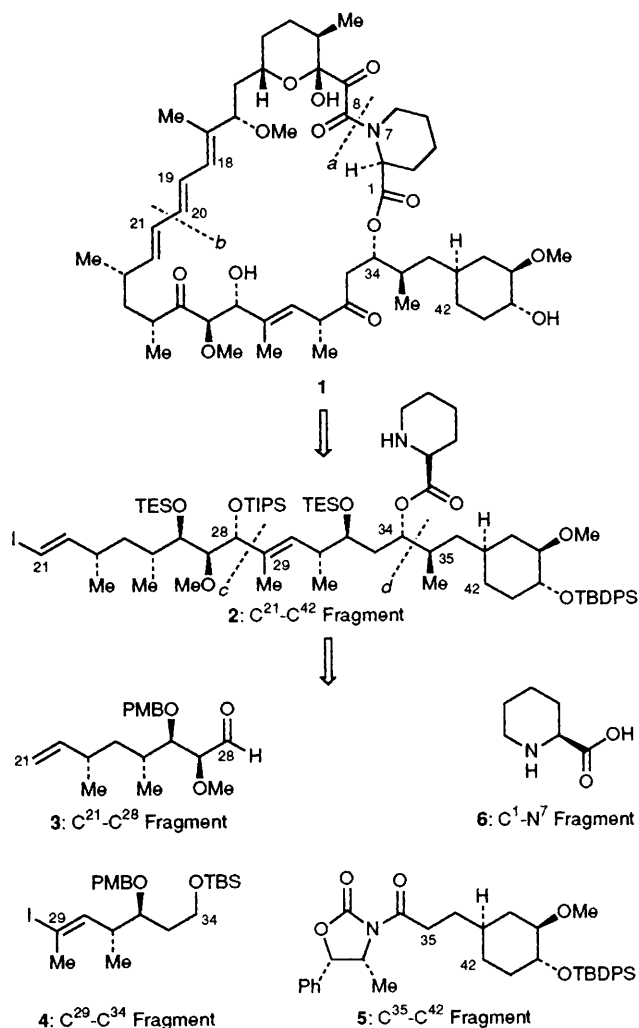
Scheme 1 Strategic bond disconnections and retrosynthetic analysis of rapamycin 1 . Definition of requisite fragments for a total synthesis.
