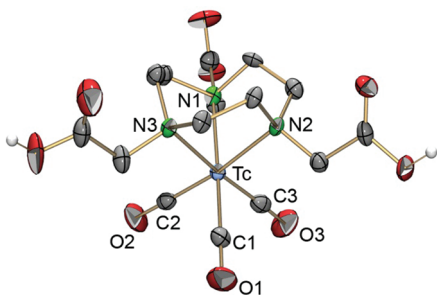
Figure 3. ORTEP 17 representation of the [^{99}\text{Tc}(\text{CO})_3(\text{nota-3H})]^+ cation [4]^+ . Thermal ellipsoids represent 50% probability. Noncarboxy hydrogen atoms are omitted for clarity. Selected bond lengths [Å] and angles [deg]: Tc–C1 1.906(3), Tc–C2 1.907(3), Tc–C3 1.910(4), Tc–N1 2.237(2), Tc–N2 2.236(2), Tc–N3 2.238(2), C1–O1 1.146(3), C2–O2 1.154(3), C3–O3 1.151(4), C1–Tc–C2 87.8(1), C1–Tc–C3 86.4(1), C2–Tc–C3 87.6(1), N1–Tc–N2 79.35(8), N1–Tc–N3 79.69(9), N2–Tc–N3 79.98(8).
