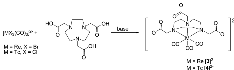
Scheme 6. Synthesis of [\text{M}(\text{nota})(\text{CO})_3]^{2-} ( \text{M} = \text{Re}, \text{Tc} )
