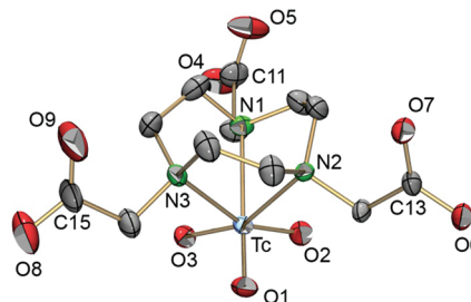
Figure 4. ORTEP 17 representation of the [^{99}\text{TcO}_3(\text{nota-0.5H})]^{1.5-} anion [5]^{1.5-} . Thermal ellipsoids represent 50% probability. Hydrogen atoms are omitted for clarity. Selected bond lengths [Å] and angles [deg]: Tc–O1 1.702(3), Tc–O2 1.713(3), Tc–O3 1.706(3), Tc–N1 2.302(4), Tc–N2 2.281(3), Tc–N3 2.296(4), O1–Tc–O2 106.5(2), O1–Tc–O3 106.6(2), O2–Tc–O3 106.2(2), N1–Tc–N2 76.2(1), N1–Tc–N3 76.4(1), N2–Tc–N3 76.6(1).
