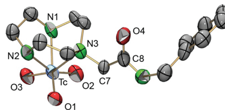
Figure 2. ORTEP 17 representation of the [^{99}\text{TcO}_3(\text{tacn-ba})]^+ [2]^+ cation. Thermal ellipsoids represent 50% probability. Hydrogen atoms are omitted for clarity. Selected bond lengths [Å] and angles [deg]: Tc–O1 1.690(4), Tc–O2 1.694(4), Tc–O3 1.693(4), Tc–N1 2.223(5), Tc–N2 2.237(4), Tc–N3 2.360(4), O1–Tc–O2 106.7(2), O1–Tc–O3 107.8(2), O2–Tc–O3 106.9(2), N1–Tc–N2 73.7(2), N1–Tc–N3 75.0(2), N2–Tc–N3 74.5(2).
