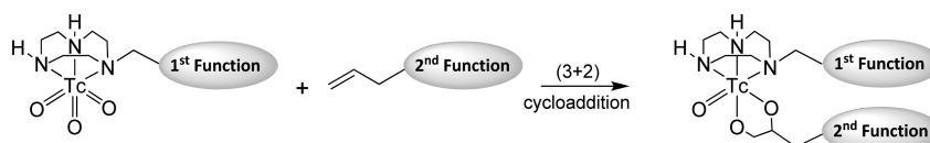
Scheme 1. Concept for the Synthesis of Site Specific Dual-Functionalized \text{fac-}\{^{99\text{m}}\text{TcO}_3\}^+ Probes Based on the BFC Approach (First Function) and (3 + 2)-Cycloaddition (Second Function)
