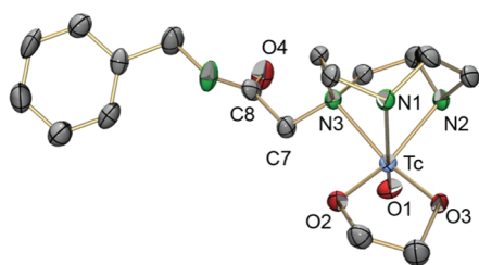
Figure 1. ORTEP 17 representation of the [^{99}\text{TcO}(\text{glyc})(\text{tacn-ba})]^+ [1]^+ cation. Thermal ellipsoids represent 50% probability. Hydrogen atoms are omitted for clarity. Selected bond lengths [Å] and angles [deg]: Tc–O1 1.664(2), Tc–O2 1.905(2), Tc–O3 1.922(2), Tc–N1 2.256(2), Tc–N2 2.142(2), Tc–N3 2.229(2), O1–Tc–O2 111.44(9), O1–Tc–O3 107.99(9), O2–Tc–O3 84.06(8), N1–Tc–N2 74.98(9), N1–Tc–N3 76.21(8), N2–Tc–N3 80.39(8).
