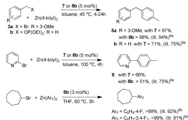
Scheme 3. Representative Cross-Coupling Reactions Catalyzed by 7 (Prepared in Situ) or 8b Compared with the Same Reactions Catalyzed by 1a (Values in Parentheses)
