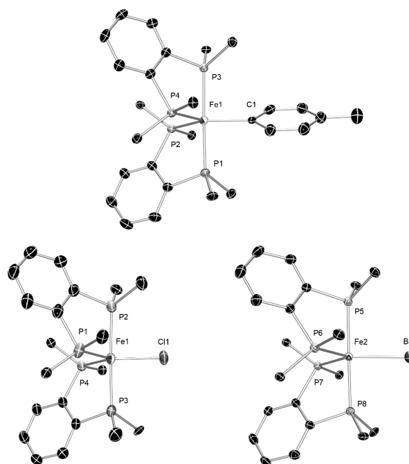
Figure 2. X-ray structures of complexes 7 (top), 8a (bottom left), and 8b (bottom right, one of two independent molecules), with the solvate molecules and all but the C ipso atoms of the PPh 2 phenyl residues omitted for clarity. The thermal ellipsoids are set at 50% probability. 14
