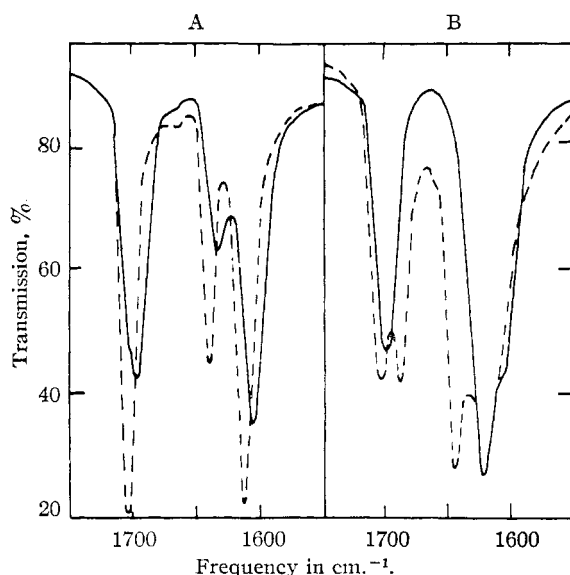
Fig. 1.—Partial infrared spectra: A, 0.7% (w/v.) solutions in chloroform, 0.5-mm. cell: —, 3-pyrrolidinyll enamine of progesterone; ---, its hydrochloride. B, Mineral oil mulls: —, 3-pyrrolidinyll enamine of progesterone; ---, its hydrochloride.
