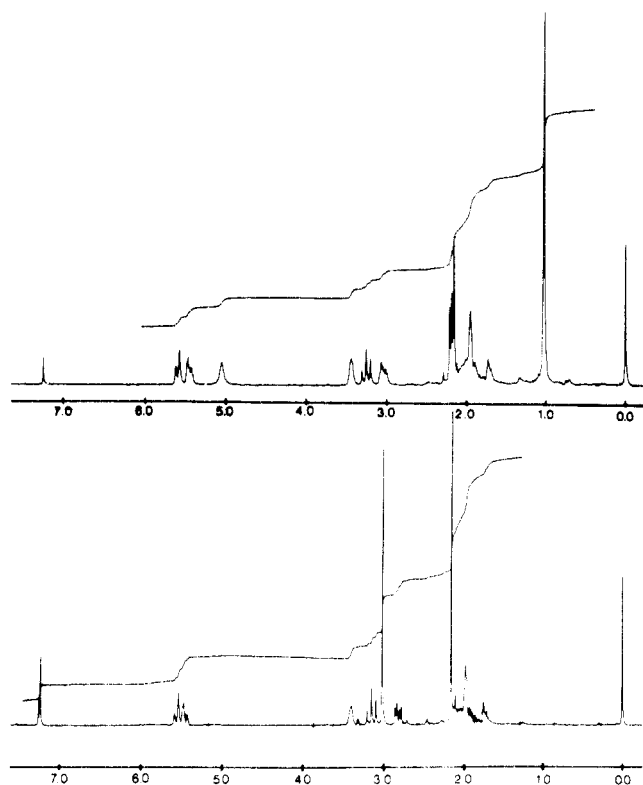
Figure 1. The 200-MHz 1 H NMR spectra of hexahydroisoquinoline 12 (bottom) and decahydrophenanthridine 25 (top) taken in CDCl 3 with chemical shift scales in ppm relative to (CH 3 ) 4 Si.
