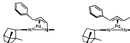
Figure 15. Two diastereomeric forms of 17 .
