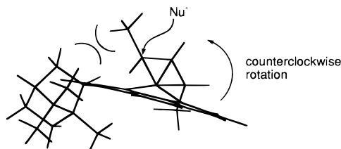
Figure 9. Steric interactions that arise from nucleophilic attack at the syn -substituted allylic C atom of anti,syn - 14 .
